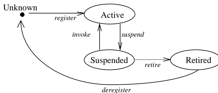
Figure 4 — Agent domain life-cycle model
