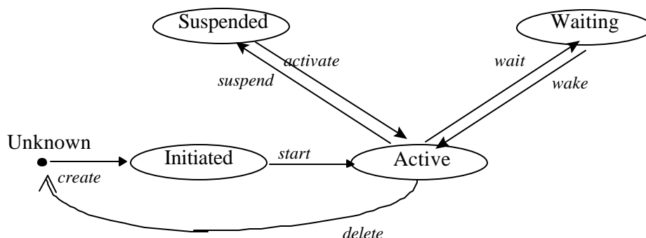
Figure 3 — AP Life-Cycle
