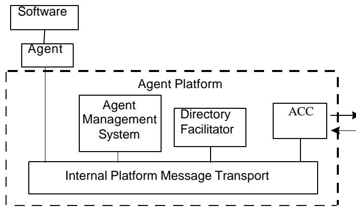
Figure 1 — Agent management reference model
