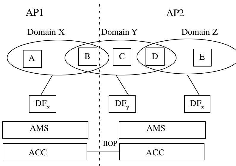
Figure 2 — Agent Platform Reference Model Fragment
